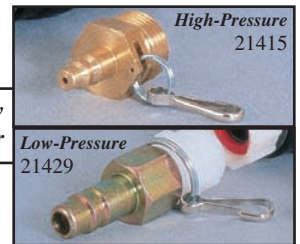
Constant-flow Connector
